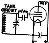
Tuned circuit serving as the tank circuit in a tuned grid-inductive plate oscillator.
